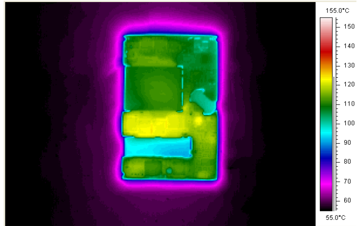
Figure 8: Thermal Image of converter at 7.6 amp load current (213W) with 55°C air flowing at the rate of 200 LFM. Air is flowing across the converter from input to output (nominal input voltage).
