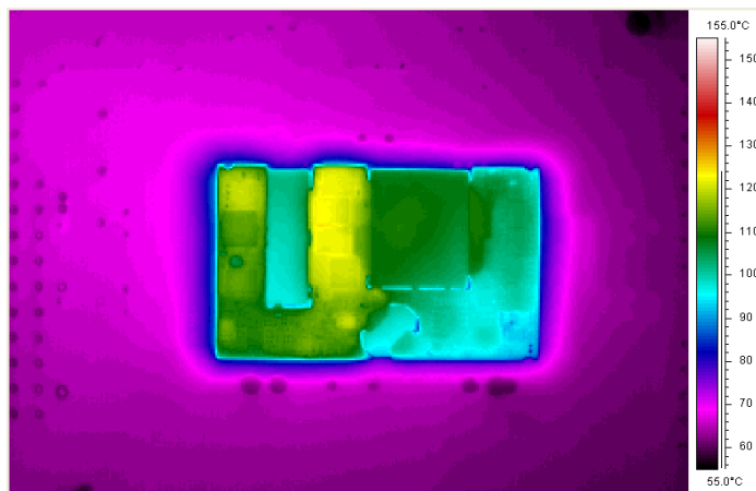
Figure 6: Thermal Image of converter at 8 amp load current (224W) with 55°C air flowing at the rate of 200 LFM. Air is flowing from pin 3 to pin 1 (nominal input voltage).
