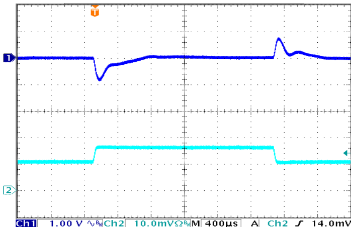
Figure 11: Output Voltage Response to Step-Change in Load Current (50%-75%-50% of Iout(max); dI/dt = 0.1A/µs). Load cap: 100µF electrolytic output capacitance. Top trace: Vout (1V/div). Bottom trace: Iout (5A/div).
