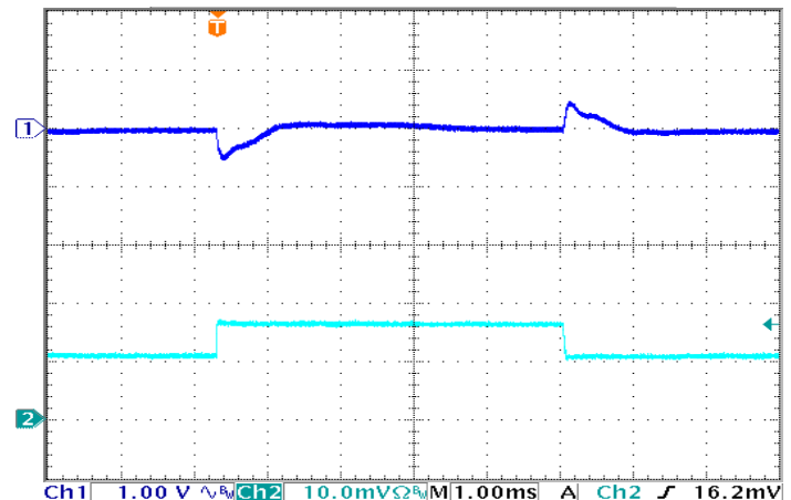
Figure 12: Output Voltage Response to Step-Change in Load Current (50%-75%-50% of Iout(max); dI/dt = 2A/µs). Load cap: 330µF electrolytic output capacitance. Top trace: Vout (1V/div). Bottom trace: Iout (5A/div).
